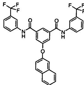
Compound # 17
